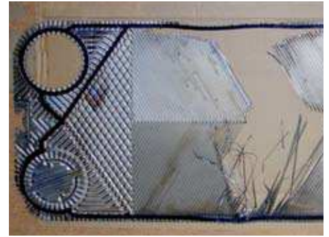
Chemical cleaning requires the right concentration, temperature and cleaning time. Otherwise, the plates can be destroyed.
