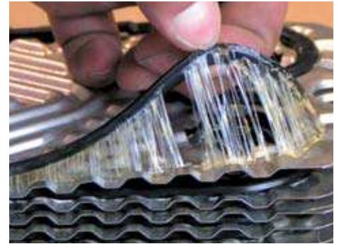
If standard glue is used on a frequently opened PHE, the gaskets may fall off, making it necessary to re-gasket after opening.
